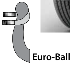
Swan-neck trailer hitch ball attached under typical European vehicle.
